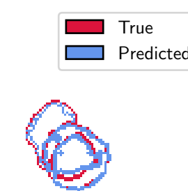
segmentations
